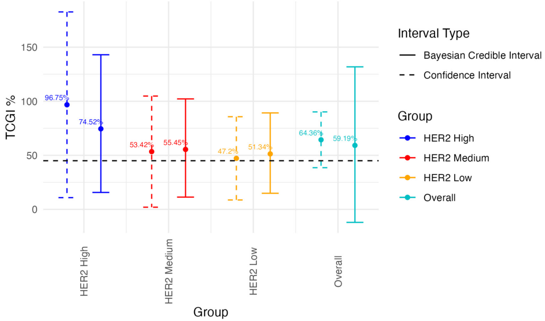
Figure 5: Bayesian Credible Intervals and frequentist Confidence Intervals for the analysis of MiniPDX data. The dots are the posterior means (Bayesian) and sample means (frequentist). The shorter the length of an interval, the more precise the statistical inference.
