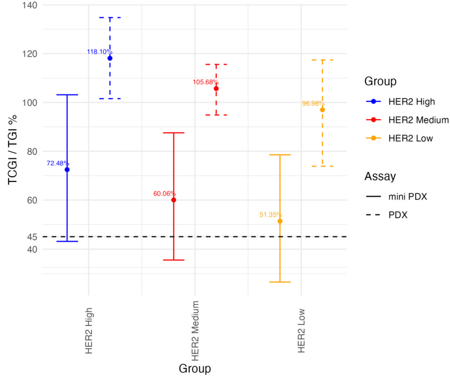
Figure 7: Bayesian credible intervals from the joint MiniPDX/PDX two-assay model for \mu_{ij} in each HER2 group (HER2 High/Medium/Low). Each color denotes a HER2 group; solid intervals are for the MiniPDX assay and dashed intervals are for the PDX assay. Dots are posterior means. The dashed horizontal line marks the 0.45 efficacy threshold.
