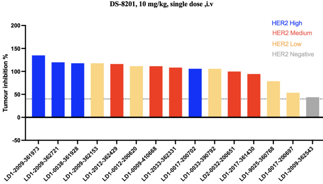
Figure 3: Tumor Inhibition (%) in PDX Models.
