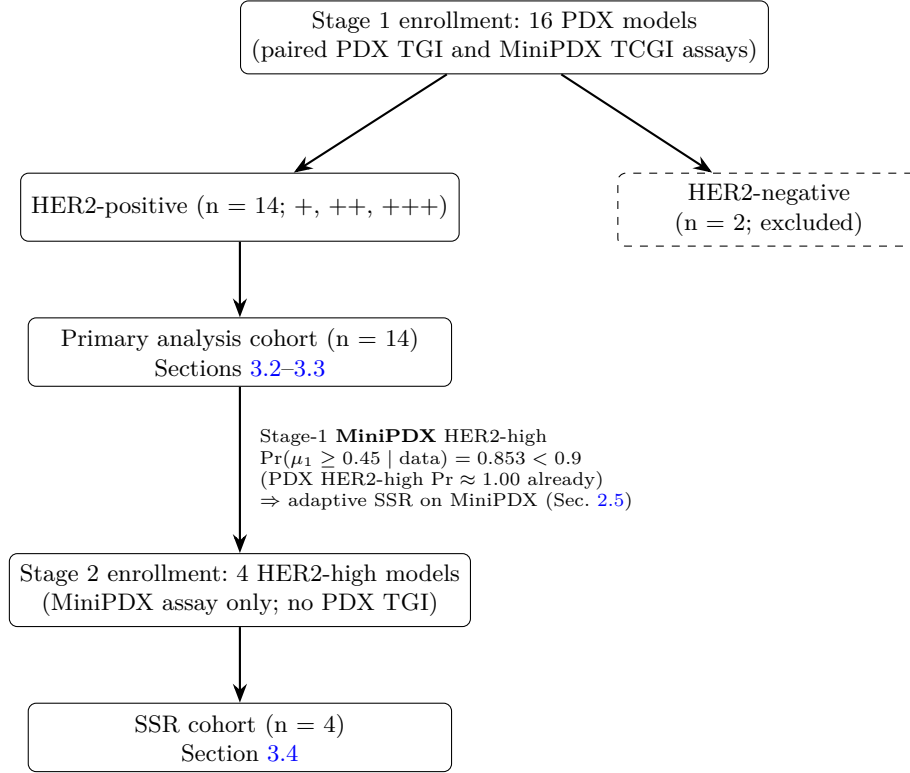
Figure 2: Sample-flow diagram for the analyses. Stage 1 enrolled 16 PDX models, each assayed on both the PDX (TGI) and MiniPDX (TCGI) platforms (Table 1, batch one). The 14 HER2-positive Stage 1 models (HER2 +, ++, +++) form the primary analysis cohort for the single-assay and two-assay hierarchical analyses; the 2 HER2-negative Stage 1 models are excluded from the hierarchical analyses because the trastuzumab deruxtecan mechanism is HER2-driven and the no-expression cohort is not expected to share the same response distribution. After Stage 1, the MiniPDX HER2-high posterior probability of efficacy was \Pr(\mu_1 \geq 0.45 \mid \text{data}) = 0.853 , below the 0.9 threshold, while the PDX HER2-high probability was already \approx 1.00 ; the SSR was therefore triggered specifically for the MiniPDX assay (Section 2.5), and Stage 2 prospectively enrolled 4 additional HER2-high models on MiniPDX only (no PDX TGI was collected for Stage 2; Table 1, batch two). These 4 Stage 2 models form the SSR cohort analyzed in Section 3.4. The excluded cohort is shown with a dashed border.
