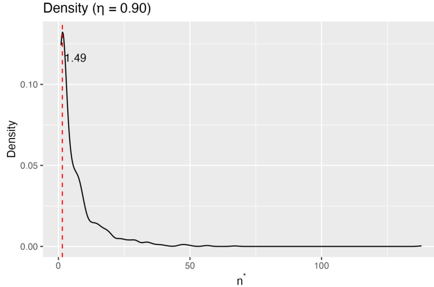
Figure 8: Density for n(\text{sim}) using Inverse Gamma prior.
