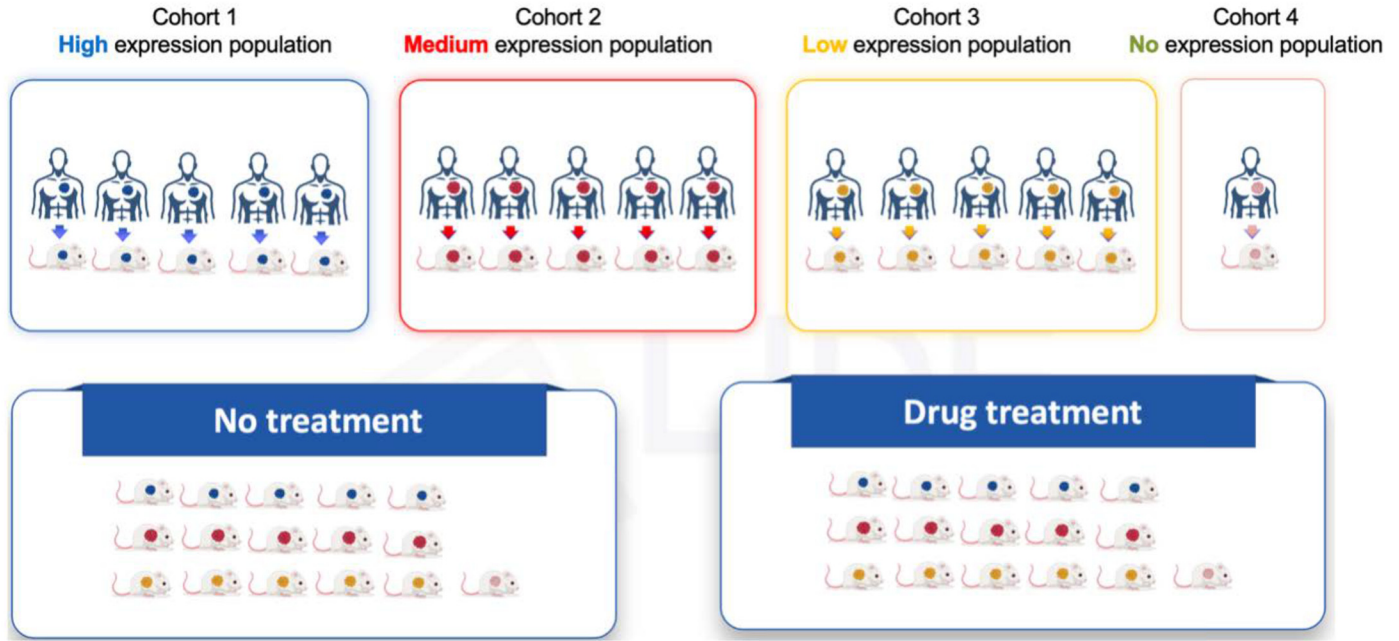
Figure 1: Fundamental Design of Mouse Clinical Trial.
