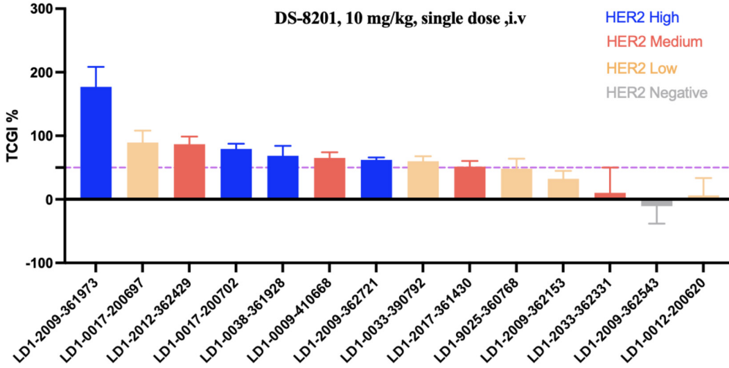
Figure 4: TCGI (%) in MiniPDX Models.
