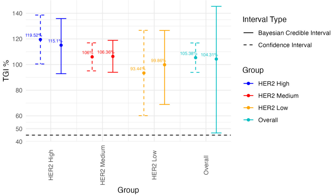
Figure 6: Bayesian Credible Intervals and frequentist Confidence Intervals for the analysis of PDX data. The dots are the posterior means (Bayesian) and sample means (frequentist). The shorter the length of an interval, the more precise the statistical inference.
