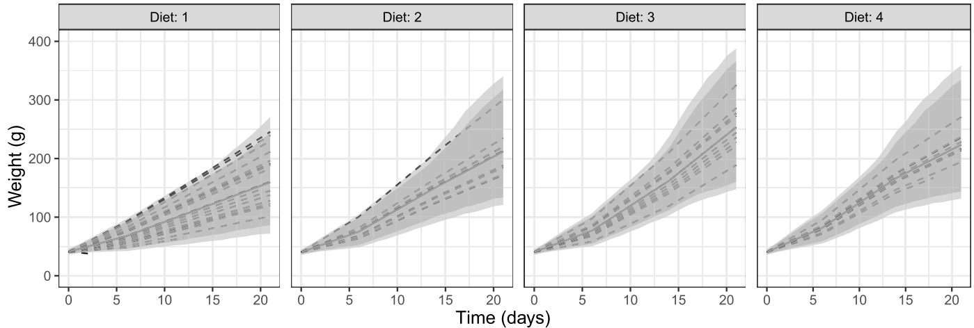
Figure 6: Fitted growing curves for all four Diet groups overlaid with the point-wise 90% and 95% confidence intervals. The solid lines are the fixed effects, and the dashed lines represent the chicks with random effects on Time.
